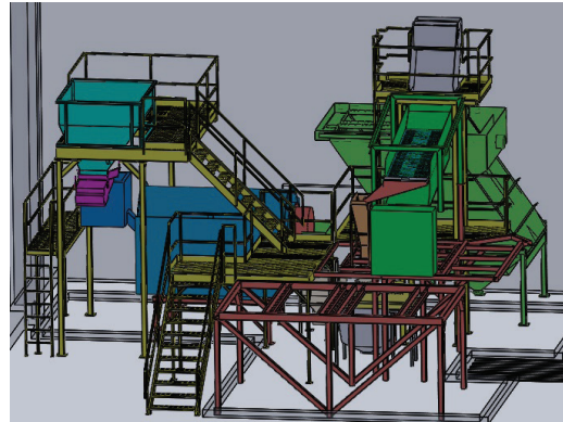
Concept: Model of Kimberlite Ore Processing Facility
