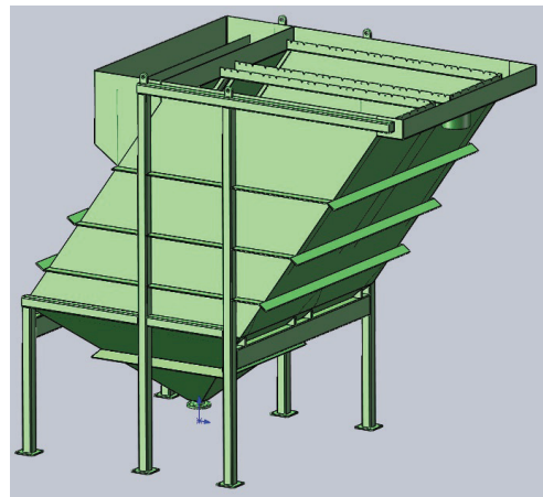
Model of Custom High-Capacity Slant Plate
